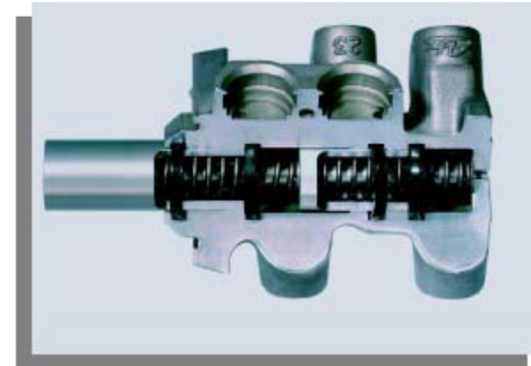
Plunger II master brake cylinder constructed of aluminum
